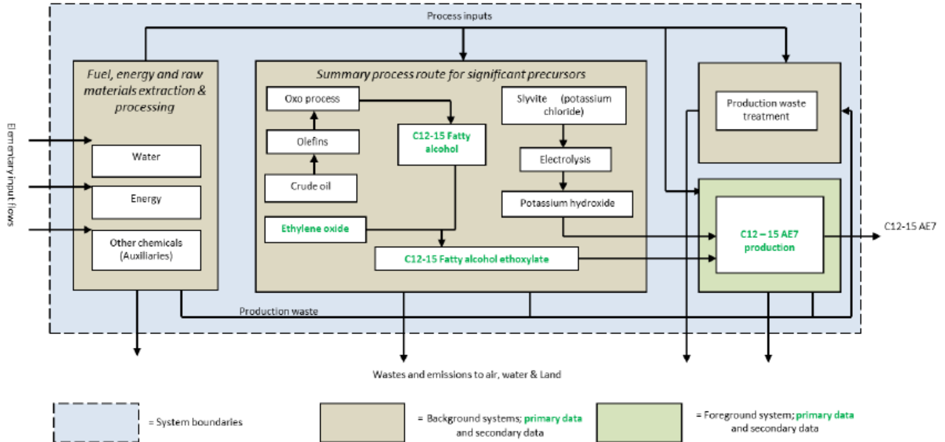
Figure1. Production process of C12-15 AE7.
